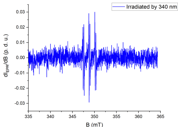
Fig. 4 EPR spectrum (X-band) of the trapped radical species between irradiated AH5 and the spin trap agent in acetonitrile. Concentrations were set to c(\text{AH5}) = 10 \text{ mM} and c(\text{N-t-butyl-}\alpha\text{-phenylnitron}) = 45 \text{ mM} . The EPR spectrum was centered at g_{\text{iso}} = 2.0065 . The hyperfine splitting structure comes from a(1 \times ^{14}\text{N}) = 1.35 \text{ mT} and a(1 \times ^1\text{H}) = 0.22 \text{ mT} .
