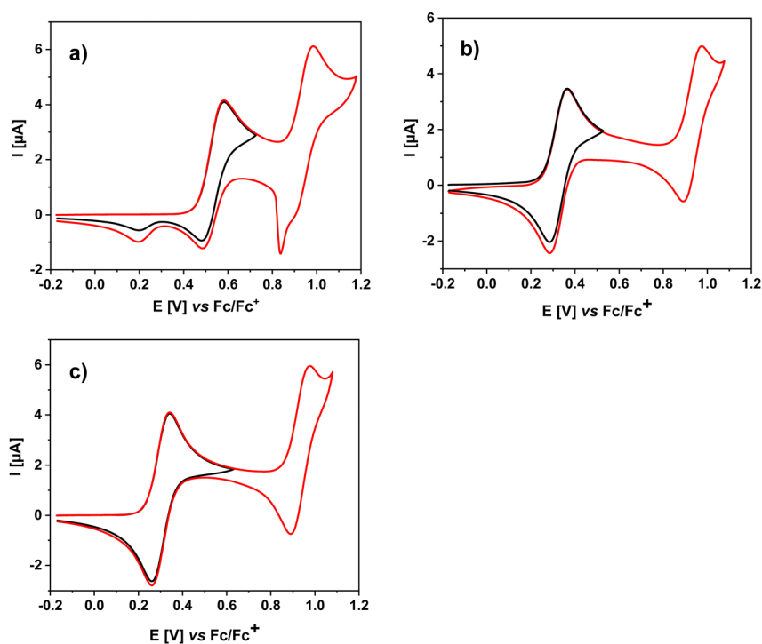
Fig. 1 Cyclic voltammograms of 1 (a), 2 (b) and 3 (c). Concentration of the studied compounds: 1 \times 10^{-3} M, electrolyte: 0.1 M Bu_4NPF_6 solution in DCM; scan rate: 50 \text{ mV s}^{-1} .
