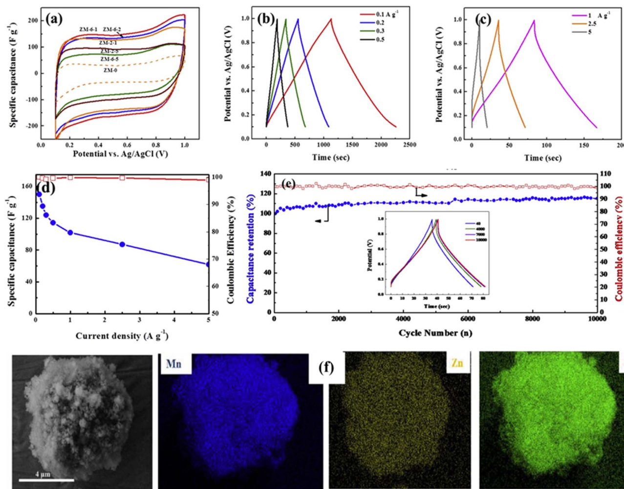
Fig. 7 Electrochemical characteristics and structural analysis of ZMO-6-1: (a) CV profiles of the synthesized samples at a scan rate of 2 \text{ mV s}^{-1} ; (b and c) GCD curves recorded at various current densities; (d) dependence of coulombic efficiency and specific capacitance on current density; (e) long-term cycling performance and coulombic efficiency over 10 000 cycles at 2.5 \text{ A g}^{-1} , with insets showing GCD profiles at the 40th, 4000th, 7000th, and 10 000th cycles. (f) SEM image and elemental mapping showcasing its structural features and elemental composition. Reproduced from ref. 92 with permission from Elsevier, copyright 2018.
