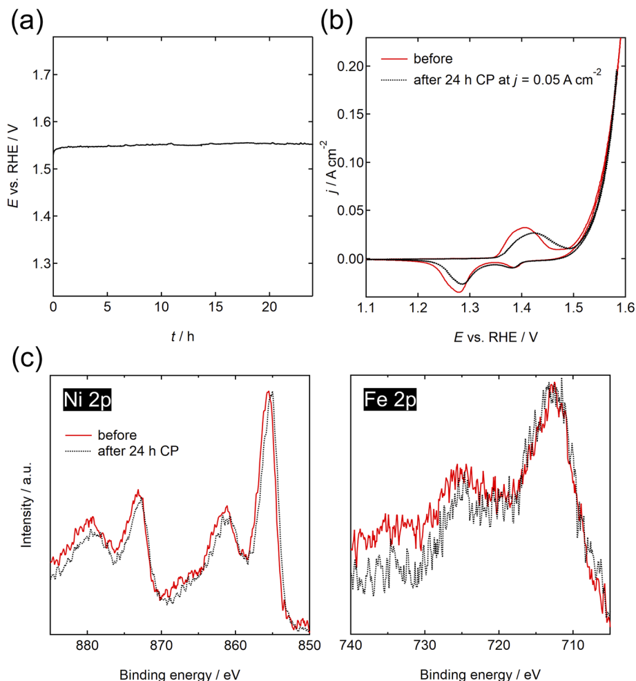
Fig. 3 (a) Potential versus time ( E - t ) curve of NiFe-LDH/NF during chronopotentiometry (CP) at a constant current density, j = 0.05 \text{ A cm}^{-2} . (b) CV plots, (c) XPS Ni 2p and Fe 2p spectra of NiFe-LDH/NF before (solid curves) and after (dashed curves) 24 h of CP at j = 0.05 \text{ A cm}^{-2} .
