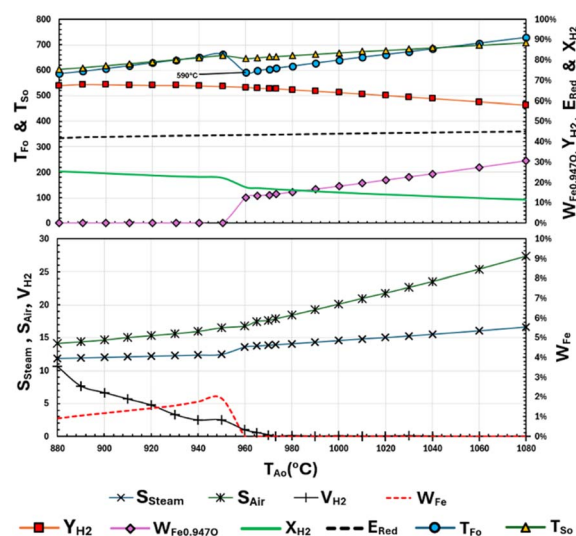
Fig. 4 Effect of T_{Ao} on hydrogen yield ( Y_{\text{H}_2} ), extent of reduction ( E_{\text{Red}} ), mass fractions of \text{Fe}_{0.947}\text{O} and Fe slip to AR ( W_{\text{Fe}_{0.947}\text{O}} , W_{\text{Fe}} ), specific steam consumption ( S_{\text{steam}} ), specific air consumption ( S_{\text{air}} ), mass fractions of \text{H}_2 in the SR gas outlet ( X_{\text{H}_2} ) and \text{H}_2 in the FR vent ( Y_{\text{H}_2} ), SR outlet temperature ( T_{So} ), and FR outlet temperature ( T_{Fo} ).
