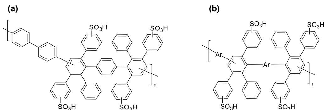
Fig. 1 Structure of (a) biphenyl-linked sulfonated phenylated polyphenylene (sPPB) and (b) Pemion®, both variations of sulfonated phenylated polyphenylenes.
