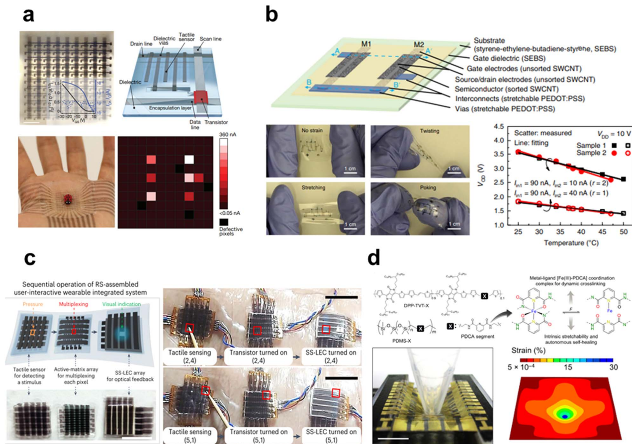
Fig. 11 Rubber-based wearable sensors based on material characteristics. Fully-stretchable skin-conformable sensors: (a) tactile sensor arrays based on CPHINE semiconductors with SEBS substrate. (b) Temperature sensor using SWCNT-based transistor on SEBS; self-healable sensors: (c) fully self-healable e-skin system using nanoconfinement of DPP-DTT with PDMS-MPU 0.4 -IU 0.6 elastomer. (d) Strain sensor utilizing metal-ligand self-healing mechanism of DPP-TVT-PDCA elastomer. Reprinted with permission from ref. 126 copyright 2018 American Association for the Advancement of Science, ref. 190 and 192 copyright 2018 & 2025 Springer Nature, and ref. 59 copyright 2019 Association for the Advancement of Science.
