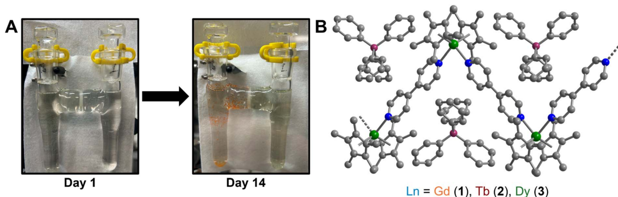
Fig. 1 (A) Glassware used for the crystallisation of \{[\text{Cp}_2^*\text{Ln}(\text{bpy})][\text{BPh}_4]\}_n (where \text{Ln} = \text{Gd} (1), \text{Tb} (2), and \text{Dy} (3)). The glass columns are bridged by a fine porosity frit, which enables crystallisation of 1–3 via slow diffusion. (B) Polymeric structure of \{[\text{Cp}_2^*\text{Dy}(\text{bpy})][\text{BPh}_4]\}_n , 3 , in a crystal of \{[\text{Cp}_2^*\text{Dy}(\text{bpy})][\text{BPh}_4]\}_n \cdot 3(\text{C}_4\text{H}_8\text{O}) . H atoms and solvent molecules in the crystal lattice have been omitted for clarity. Green, blue, grey, and purple spheres represent Dy, N, C, and B atoms, respectively. Select distances (Å) and angles ( ^\circ ): Ln–C Cp* : 2.676(10)–2.743(24) (1); 2.633(12)–2.747(26) (2); 2.649(19)–2.711(21) (3); Ln–Cnt: 2.423 (1); 2.395 (2); 2.392 (3); Ln–N: 2.488(6) (1), 2.447(7) (2), 2.444(5) (3); Cnt–Ln–Cnt: 131.7 (1), 132.3 (2), 133.0 (3); N–Ln–N: 91.1(2) (1); 91.5(2) (2), 90.6(2) (3); Ln–Ln–Ln: 91.7(1) (1), 91.3(1) (2), 91.8(1) (3); Ln–N–N–Ln: 180.0(1) (1–3); Ln–B–Ln–B: 180.0(1) (1–3) (where B is the boron atom of the (\text{BPh}_4)^- counteranion); Ln–Ln–Ln–Ln: 180.0(1) (1–3).
