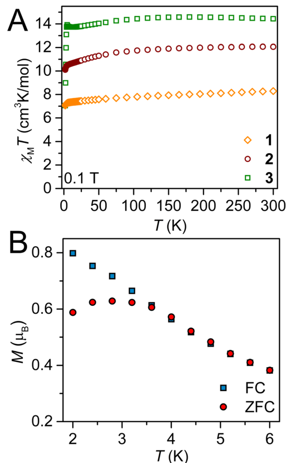
Fig. 3 (A) Variable-temperature dc magnetic susceptibility data for \{[Cp_2^*Ln(bpy)][BPh_4]\}_n , where Ln = Gd, 1 (orange diamonds), Tb, 2 (maroon circles), Dy, 3 (green squares), collected under a 0.1 T applied dc field. (B) Plot of magnetisation vs. temperature for 3 during field-cooled (blue squares) and zero-field-cooled (red circles) measurements depicting the thermoremanent magnetization. The divergence at 4 K is indicative of magnetic blocking.
