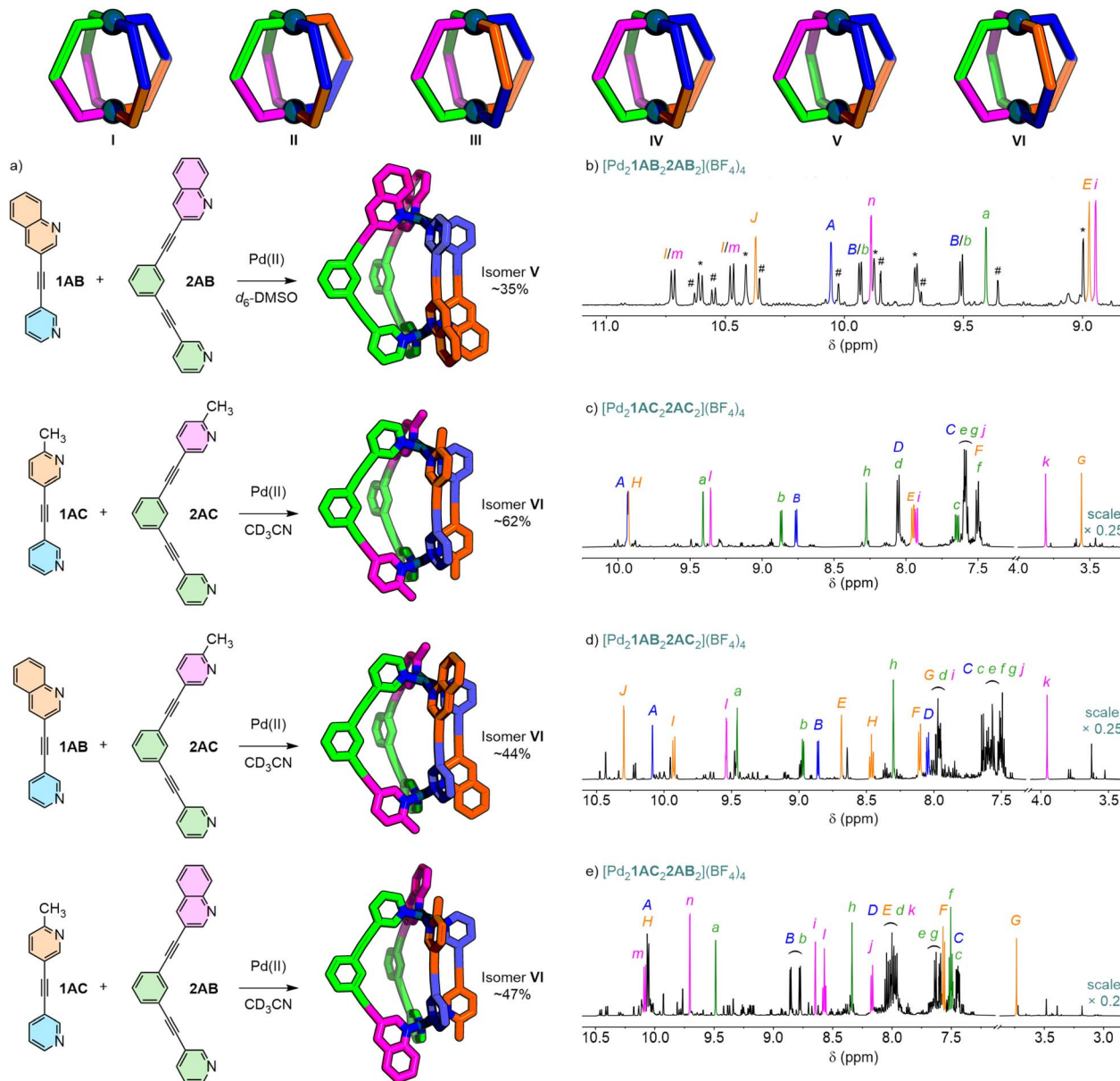
Fig. 8 (a) The selective formation of particular isomers of Pd 2 L A L B 2-type cages (GXN2-xTB geometry-optimised models shown) from combinations of ligands 1AB / 1AC and 2AB / 2AC was observed. Partial 1 H NMR spectra (600 MHz, 298 K) of (b) [Pd 2 1AB 2 2AB ] 2 (BF 4 ) 4 (d 6 -DMSO) with peaks assigned to major isomer V labelled (# = minor isomer; * = [Pd 2 2AB 4 ] 4+ ); and (c) [Pd 2 1AC 2 2AC ] 2 (BF 4 ) 4 , (d) [Pd 2 1AB 2 2AC ] 2 (BF 4 ) 4 , and (e) [Pd 2 1AC 2 2AB ] 2 (BF 4 ) 4 (all CD 3 CN) with peaks assigned to major product, isomer VI, labelled.
