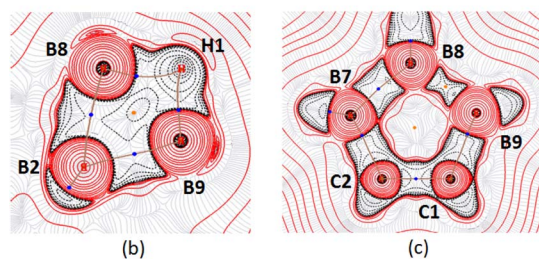
Fig. 8 (a) Selected NBO of 5 showing the 3c–2e interaction of B8–H1–B9 (isocontour values: \pm 0.045 [e bohr ^{-3} ] ^{1/2} ). Contour-line diagram of the Laplacian of the electron density along (b) B8–H1–B9 and (c) B7–B8–B9 planes in 5 .
