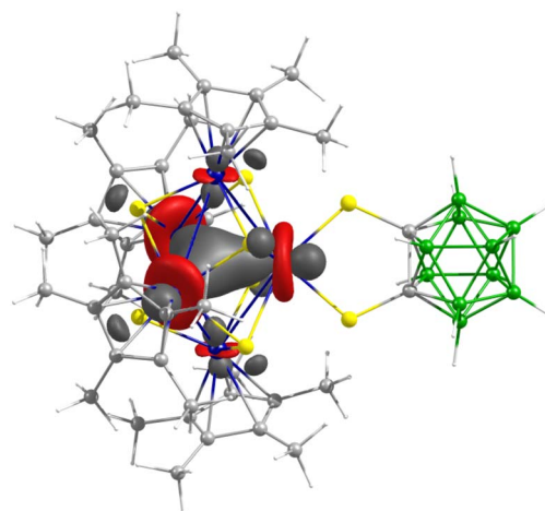
Fig. 4 HOMO of 2 showing 3c–2e equatorial trititanium interactions (isocontour values: ±0.045 [e bohr -3/2 ]).
