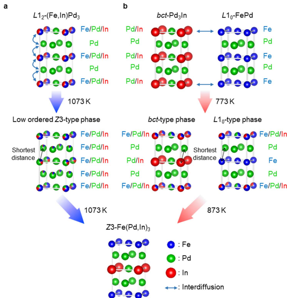
Fig. 6 (a and b) Illustrations of the formation processes for the Z3\text{-Fe(Pd,In)}_3 phase obtained from the L1_2\text{-(Fe,In)Pd}_3 (a) and L1_0\text{-FePd/bct-Pd}_3\text{In} (b) diphases, which are the intermediate structures formed from \text{FePd}_3\text{In} and \text{PdIn}_x\text{Fe} NPs, respectively.
