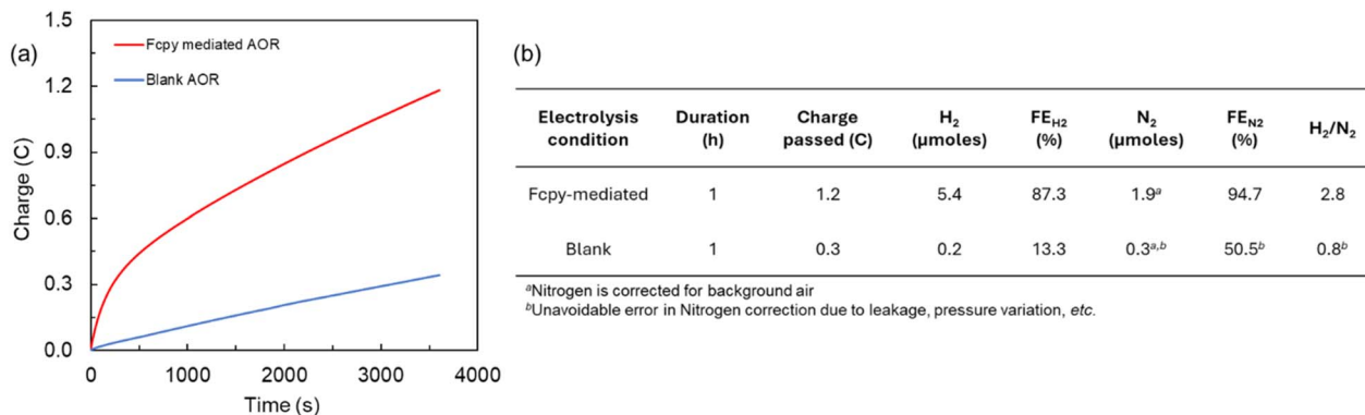
Fig. 3 (a) Constant potential electrolysis at 0.28 V (vs. Fc +0 ) for the same duration without (blue) and with (red) 1 mM Fcpy using 1 × 1 cm 2 carbon-cloth as working electrode. Experimental conditions: 100 mM TBAF as supporting electrolyte in acetonitrile, 3-electrode setup in an undivided cell, 298 K; (b) summary of product quantification results after electrolysis with an average of three measurements.
