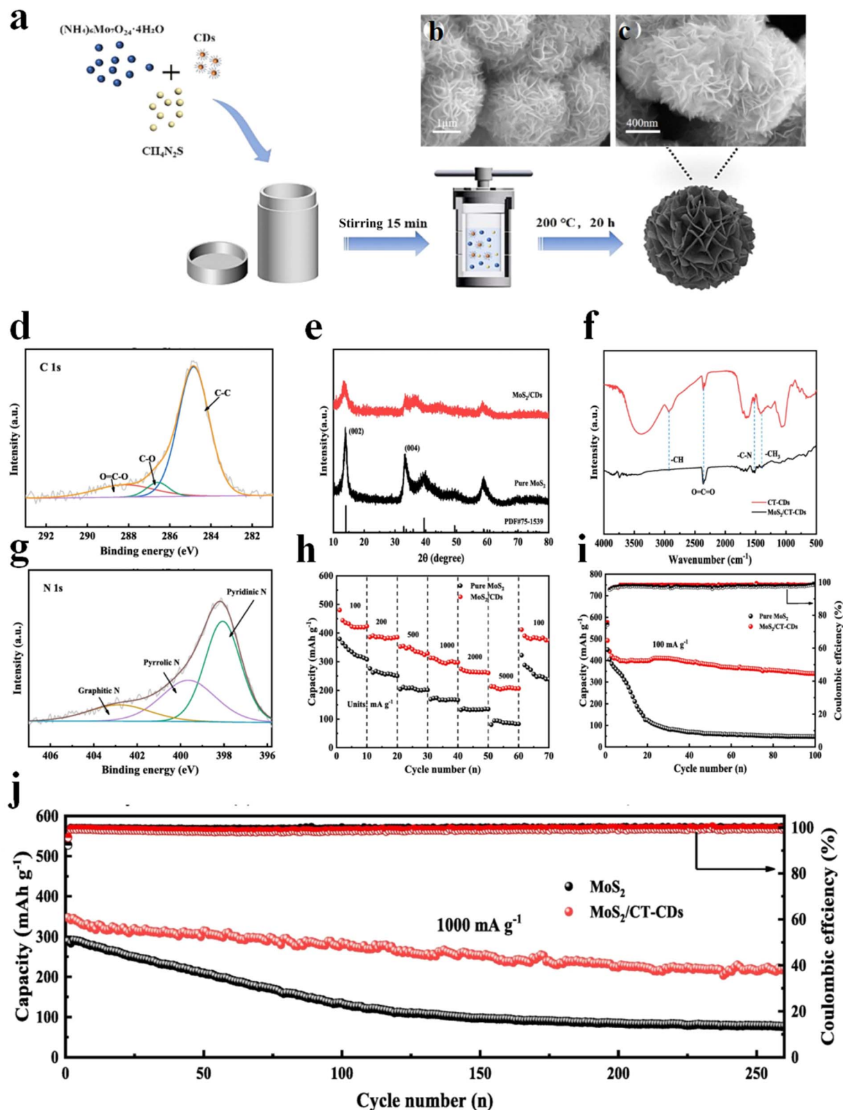
Fig. 8 CT-CDs derived from chitin: (a) schematic illustration of the synthesis process of \text{MoS}_2/\text{CT-CDs} ; (b and c) SEM images of \text{MoS}_2/\text{CT-CDs} ; (d) C 1s XPS spectrum; (e) XRD pattern; (f) FT-IR spectrum; (g) N 1s XPS spectrum; (h) rate properties of \text{MoS}_2 and \text{MoS}_2/\text{CT-CDs} ; (i) cycle properties of \text{MoS}_2 and \text{MoS}_2/\text{CT-CDs} ; (j) long-term cycle stability of \text{MoS}_2 and \text{MoS}_2/\text{CT-CD} . Reproduced with permission. 55 Copyright 2024, Elsevier.
