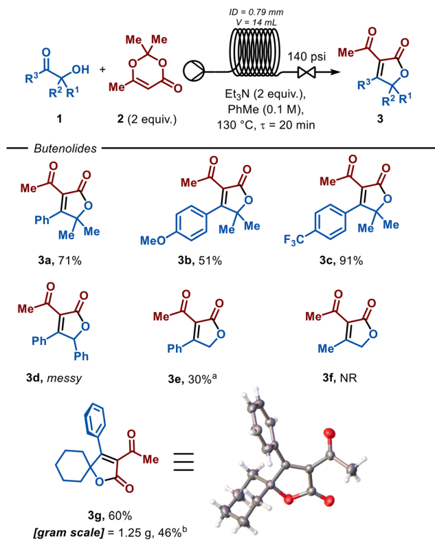
Fig. 2 Scope of butenolides. Reaction conditions: a solution of 1 (0.25 mmol), 2 (2 equiv.), and \text{Et}_3\text{N} (2 equiv.) in \text{PhMe} (0.1 M) was pumped at 0.7\text{ mL min}^{-1} through a 14 mL HPFA tubing (ID 0.79 mm) and heated at 130^\circ\text{C} . Isolated yield by chromatography column. a Fed-batch procedure. b Purified by crystallization. NR = no reaction.
