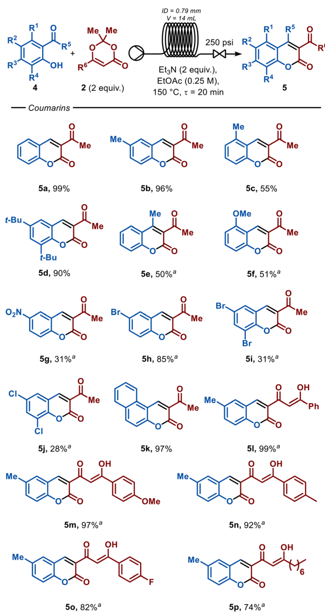
Fig. 3 Scope of coumarins. Reaction conditions: a solution of 4 (0.50 mmol), 2 (2 equiv.), and \text{Et}_3\text{N} (2 equiv.) in \text{EtOAc} (0.25 M) was pumped at 0.7\text{ mL min}^{-1} through a 14 mL HPFA tubing (ID 0.79 mm) and heated at 130^\circ\text{C} . Isolated yield by chromatography column. a THF used as the solvent due to poor solubility in \text{EtOAc} . NR = no reaction.
