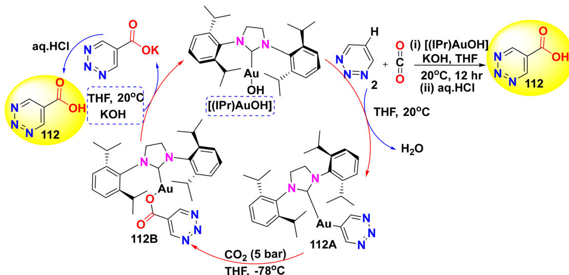
Scheme 45 Proposed mechanism for the formation of triazine carboxylic acid.
