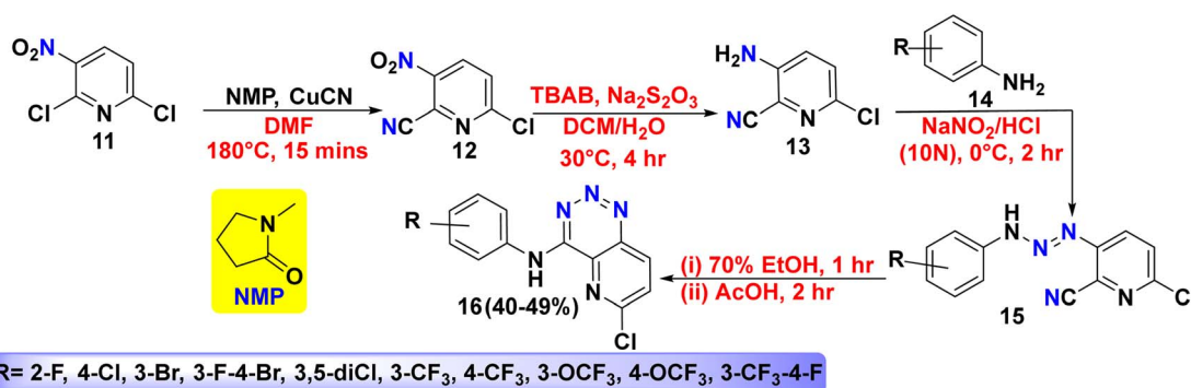
Scheme 7 Synthetic strategy for the constitution of fused pyrido-triazines.
