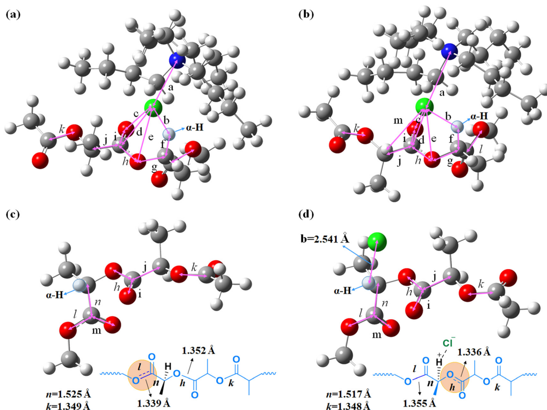
Fig. 4 M06-2X/6-21G optimized geometries of TBACl and the chain segment of (a) PLA (R,S) or (b) PLLA (S,S). M06-2X/6-21G optimized geometries of (c) PLA (R,S) and (d) PLA (R,S) affected by chloride ions in TBACl. To enhance the observation of structural alterations, the chain segment orientation of PLA (R,S) in (c) and (d) is reversed relative to that observed in (a).
