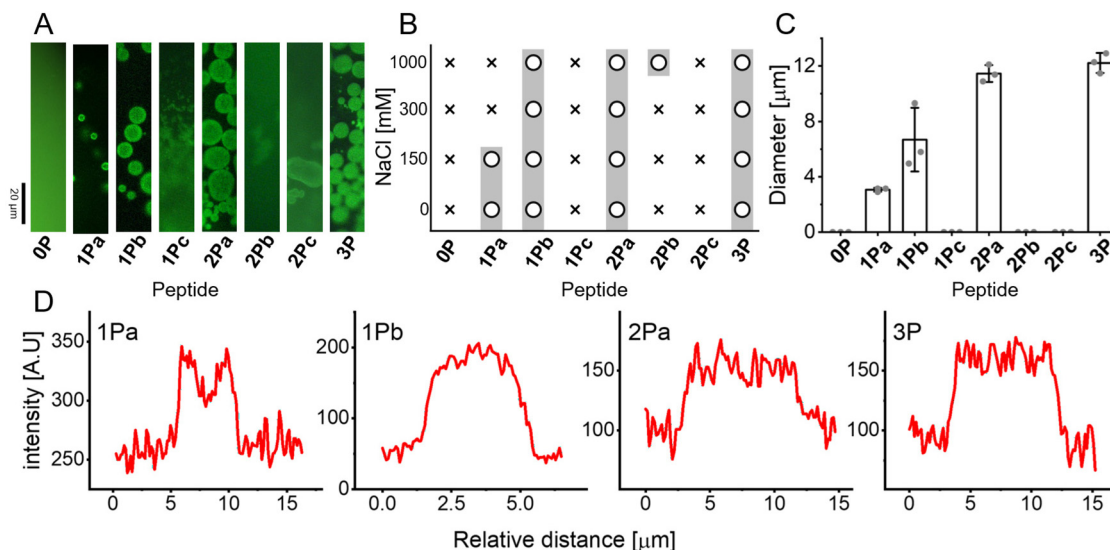
Fig. 4 (A) Fluorescence microscopy of the peptide library. Only 1Pa, 1Pb, 2Pa and 3P made condensates. (B) The dependence of peptides condensates on ionic strength. 'O' with grey background: condensates formation; 'X': No condensates formation. X axis is the peptide library, Y axis is NaCl concentration in mM. (C) The maximum diameter size of the condensates of the different peptides. (D) Cross-section analysis of condensates of the peptides that underwent condensation. X axis is the position within the cross-section of the condensate in μm. The 0 μm position was defined as the starting point of the measurement. Y axis is the intensity of each position. 1Pa has higher fluorescence intensity around the condensate edges while in the other peptides, the intensity is uniform.
