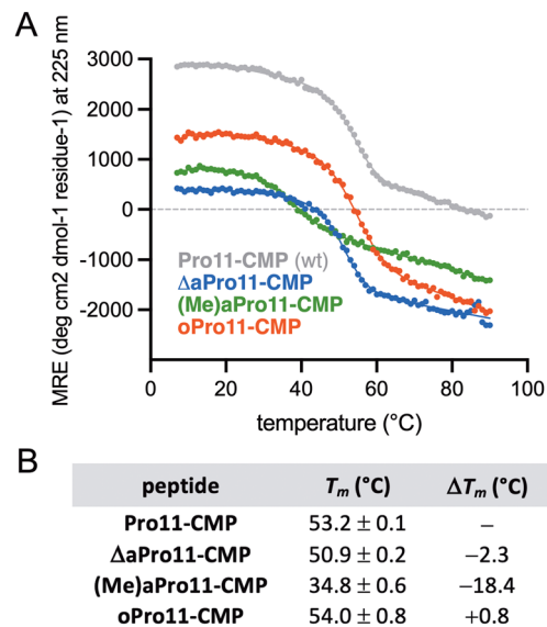
Fig. 3 Thermal denaturation of CMPs at 150 μM in aq PBS (pH 7.4). (A) Representative plot of MRE at 225 nm as a function of temperature determined by CD. (B) Melting temperatures ( T_m ) and change in T_m ( \Delta T_m ) relative to Pro11-CMP derived from non-linear regression. T_m values represent the mean and standard deviation from two separate experiments.
