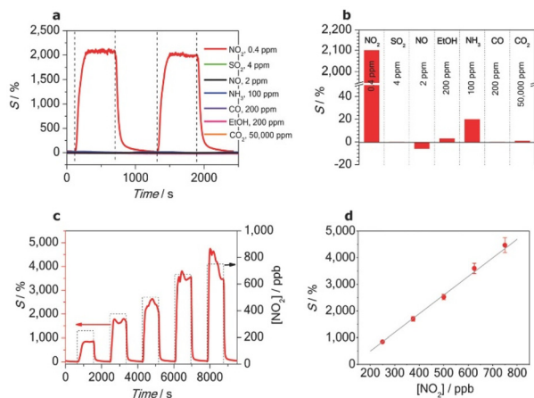
Fig. 7 en-APTAS 1 functionalized \text{SnO}_2 NW sensor measured under solar illumination ( 85\ \text{mW cm}^{-2} ). (a) Pulses of 0.4\ \text{ppm} \text{NO}_2 , \text{SO}_2 ( 4\ \text{ppm} ), \text{NO} ( 2\ \text{ppm} ), \text{NH}_3 ( 100\ \text{ppm} ), ethanol ( 200\ \text{ppm} ), \text{CO} ( 200\ \text{ppm} ) and \text{CO}_2 ( 50\ 000\ \text{ppm} ). (b) Summary of sensitivities towards the tested gases. (c) Sensing response vs. different \text{NO}_2 concentrations ranging from 250 to 750\ \text{ppb} in synthetic air. (d) Linear behaviour of the sensor response with different \text{NO}_2 concentrations. Reproduced from ref. 48 with permission from Wiley, copyright 2014.
