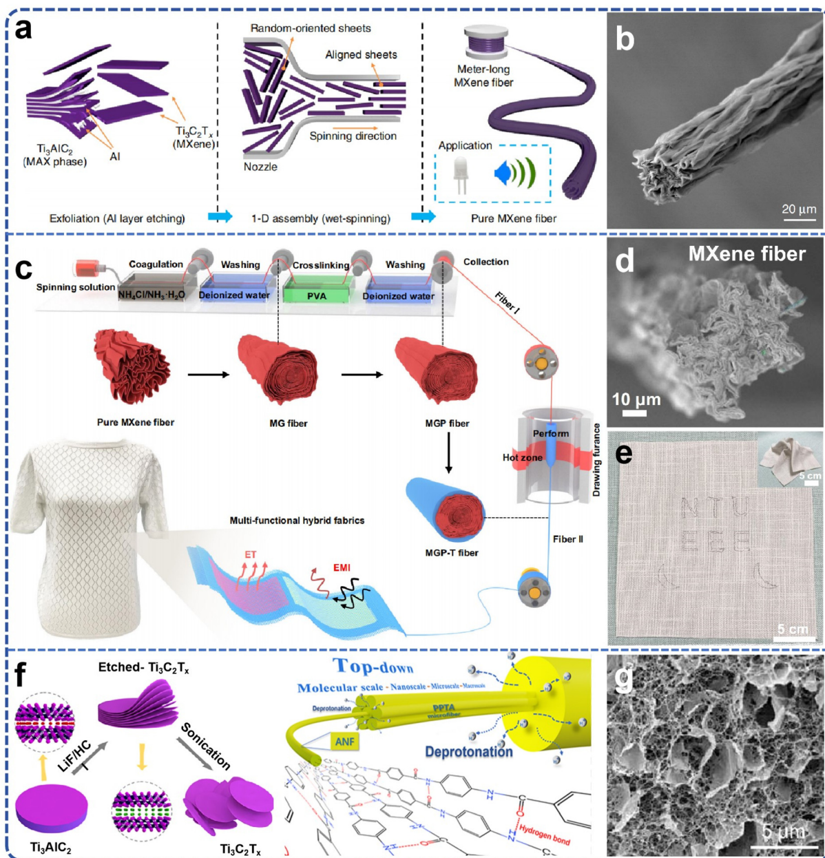
Fig. 6 (a) Schematic illustration of the reconstruction of MXene single layers into MXene fibers; (b) SEM images of Ti_3C_2T_x MXene fiber. Reproduced from ref. 23 with permission from Nature, copyright 2020. (c) Fabrication of MGP-T fiber via continuous wet spinning and thermal drawing, and the formation of MXene-based textiles; (d) pure MXene fibers; (e) designed patterns woven into the cotton cloth under complex deformations (inset). Reproduced from ref. 22 with permission from Nature, copyright 2022. (f) ANF diagram of MXene preparation and stripping from aramid fibers; (g) SEM image of freeze-dried hydrogel, presenting a 3D ANF network with evenly distributed MXene nanosheets. Reproduced from ref. 75 with permission from American Chemical Society, copyright 2022.
