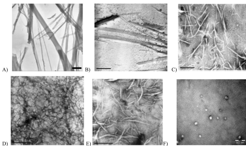
Fig. 2 TEM images of hydrogel (A) 0.4% (w/v) Ac-L-Phe-L-Phe-L-Ala-NH 2 in water. (B) Hydrogel with liposomes at a 5 : 1 molar ratio, stained with Pd. (C) Hydrogel with liposomes at a 5 : 1 ratio, stained with pWk; magnification 8000×. scale = 1 μm. (D) with BSA; (E) with liposome BSA; stained with pWk; magnification 16000×. scale = 1 μm; (F) liposomes alone, scale = 500 nm.
