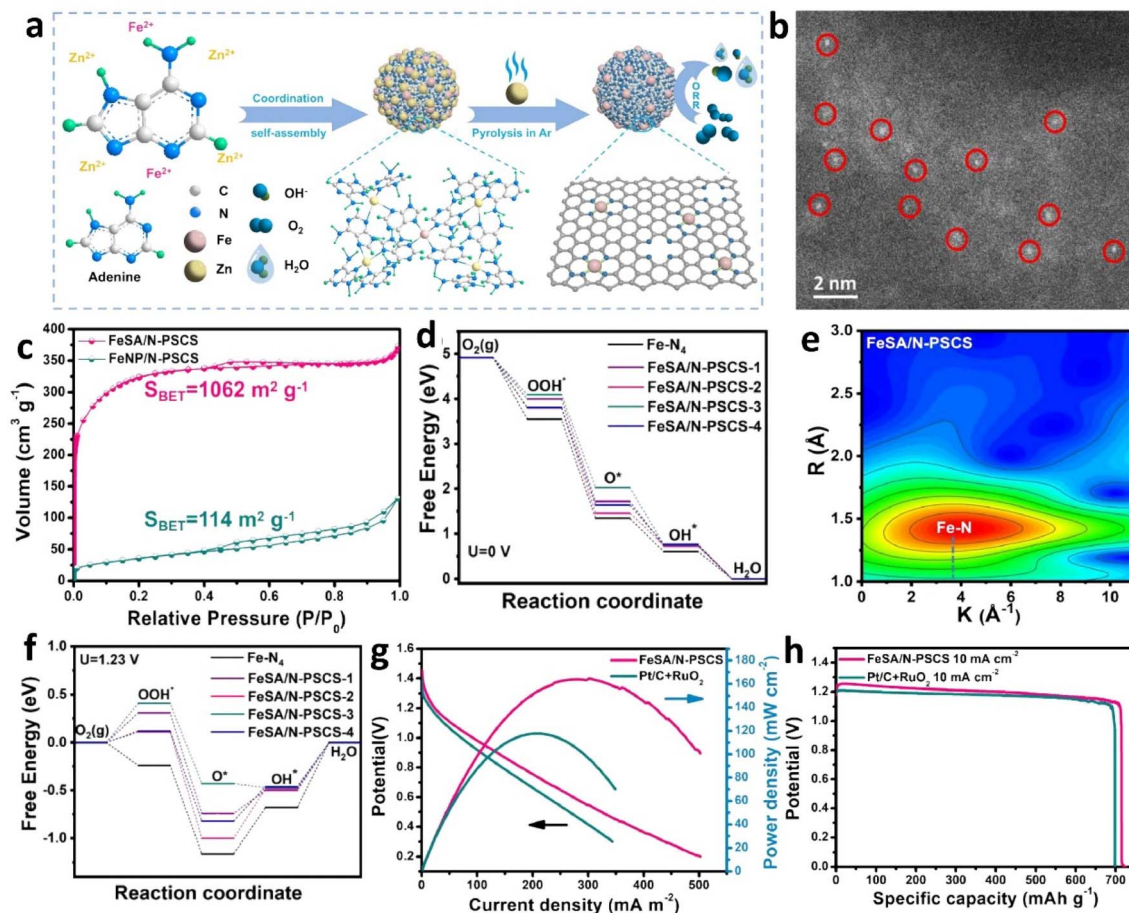
Fig. 3 (a) Synthesis of an FeSA/N-PSCS catalyst. (b) AC-HAADF-STEM image. (c) N 2 adsorption-desorption isotherms. (d) Gibbs free energy at U = 0 \text{ V} for Fe-N 4 and FeSA/N-PSCS-X. (e) Wavelet transforms of EXAFS signals. (f) Gibbs free energy at U = 1.23 \text{ V} for Fe-N 4 and FeSA/N-PSCS-X. (g) Polarization and power density curves of ZABs with FeSA/N-PSCS and Pt/C + RuO 2 catalysts. (h) Discharge-specific capacity of ZABs at 10 \text{ mA cm}^{-2} . Reproduced with permission from ref. 25 Copyright 2024, Elsevier.
