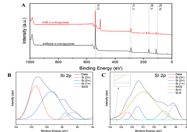
Fig. 3 (A) X-ray photoelectron spectroscopy (XPS) spectra of synthesized silica nanoparticles (SNP) of both with and without \kappa -carrageenan including the deconvolution of the Si 2p region of the XPS for (B) without \kappa -carrageenan and (C) with \kappa -carrageenan.
