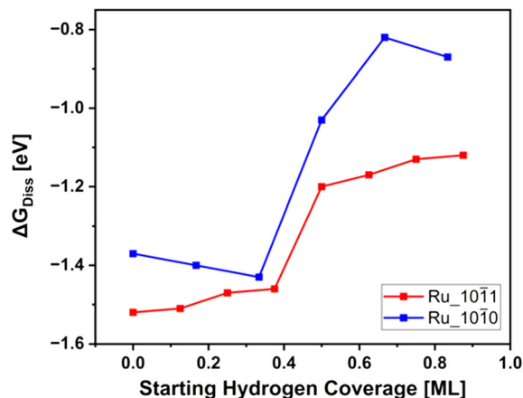
Fig. 1 H_2 direct dissociation energy ( \Delta G_{Diss} ) in eV as a function of the starting atomic hydrogen coverage ( i.e. , the coverage before the dissociation reaction) reported in monolayers (MLs) for the Ru (10 \bar{1}1 ) and (10 \bar{1}0 ) surfaces. Energies are reported at 0 K with ZPE corrections.
