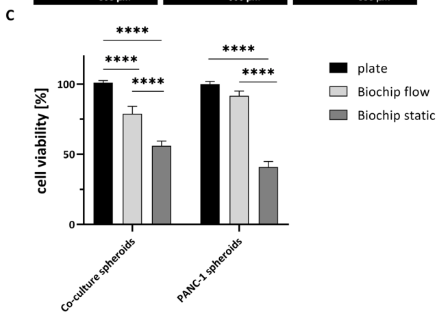
Fig. 2 Cultivation of spheroids on the biochip. (A) Co-culture spheroids and PANC-1 spheroids loaded into the microcavities of the biochip. Images are taken via bright field microscopy after loading of the spheroids. Scale is 1000\ \mu\text{m} . (B) If staining of 3D PANC-1 and co-culture spheroids after 72 h cultivation on the biochip shown as maximum intensity projection (MIP) of a Z-stack. DAPI-staining of nuclei (blue); staining of the proliferation marker Ki67 (green); staining of fibroblast marker \alpha\text{-SMA} (purple); merging of all three channels. Scale bar is 500\ \mu\text{m} . (C) Investigation of cell viability of 3D spheroids after 72 h cultivation on biochip either under flow or static conditions in comparison to the cultivation in a 96-well plate. Error bars indicate the standard errors of the mean of at least three independent experiments, with **** = p \leq 0.0001 .
