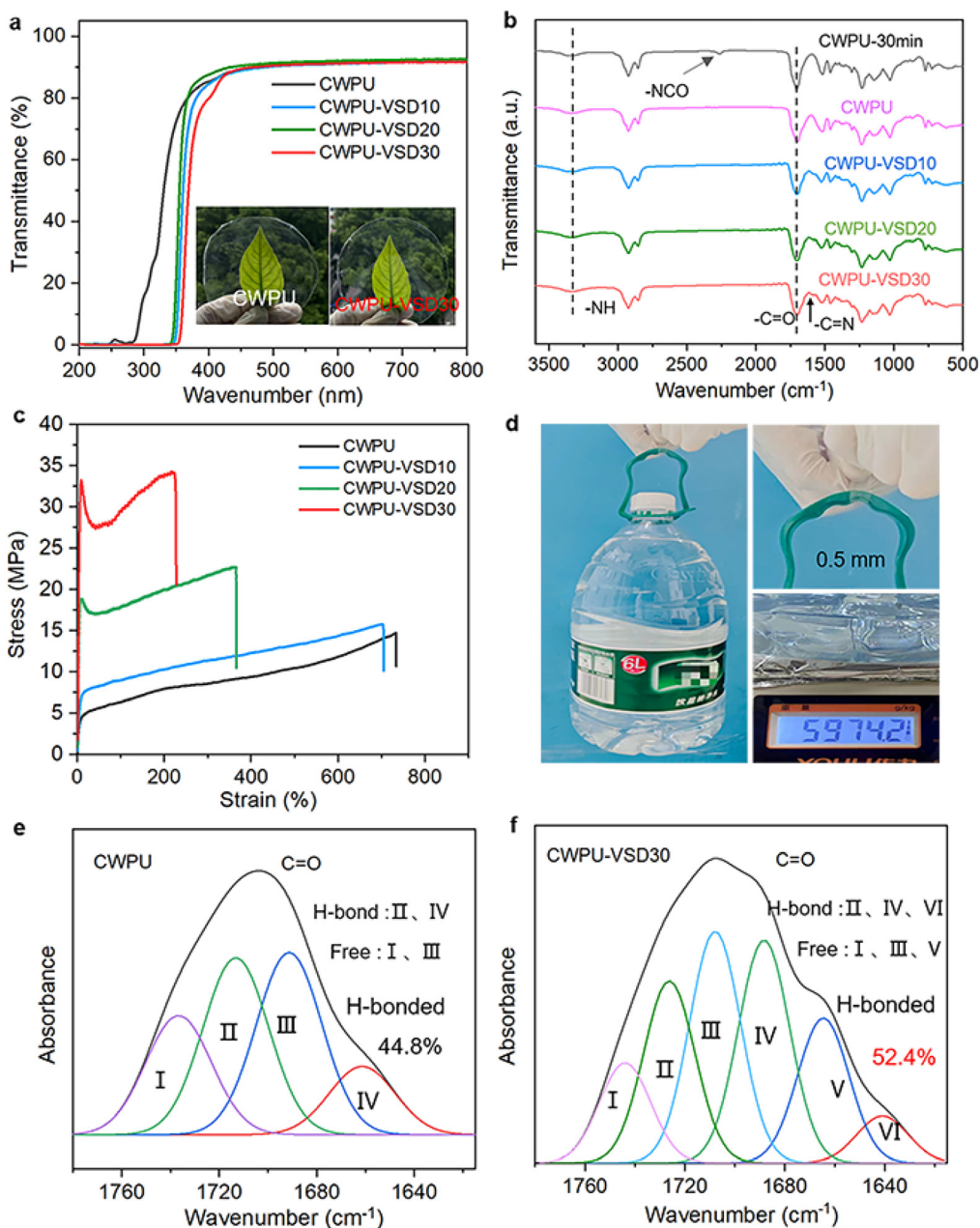
Fig. 2 (a) UV-vis transmittance spectra. Inset: photos of the CWPU and CWPU-VSD30 (colorless and transparent) films. (b) FTIR spectra of CWPU and CWPU-VSD samples. (c) Stress-strain curves of CWPU and CWPU-VSD films. (d) Photos showing that CWPU-VSD30 thin sheet can lift a weight of about 6 kg. Curve-fitting results of the carbonyl region in the FTIR spectra for (e) CWPU and (f) CWPU-VSD30.
