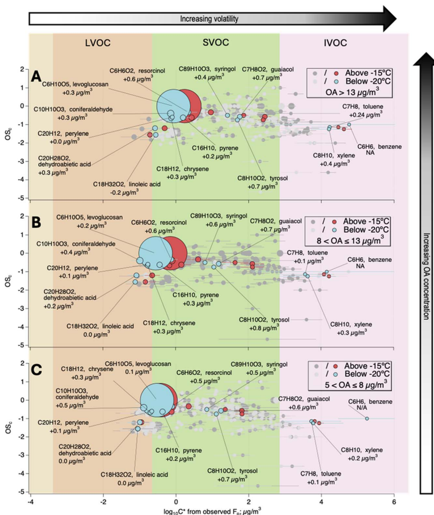
Fig. 3 The oxidation state of carbon in the detected ions ( OS_c ) versus the average effective saturation mass concentration ( C^* ) as a function of OA concentrations ( i.e. , vertical panning) and temperature (within each panel). The average \log_{10} C^* is shown for three ranges of OA concentrations: >13 \mu\text{g}/\text{m}^3 (A), 8\text{--}13 \mu\text{g}/\text{m}^3 (B) and 5\text{--}8 \mu\text{g}/\text{m}^3 (C). Compounds associated with known sources of OA emissions in Fairbanks are annotated and shown in blue (below -20^\circ\text{C} ) and red (above -15^\circ\text{C} ) colours. The value written under each ion is the \Delta\log_{10} C^* , i.e. , the difference between the average \log_{10} C^* of each ion at the two temperature ranges; a positive \Delta\log_{10} C^* indicates an increase in volatility above -15^\circ\text{C} . Data points are sized by abundance normalised to the concentration of levoglucosan. The background delineates data points into volatility classes based on the volatility-basis set. 4,9 Error bars show one standard deviation.
