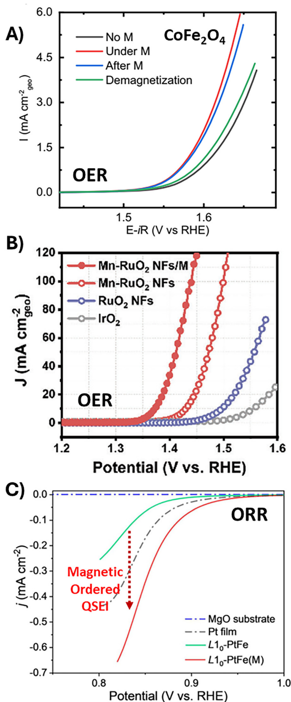
Fig. 9 Linear sweep voltammetry curves of: (A) ferrimagnetic \text{CoFe}_2\text{O}_4 at a scan rate of 10 \text{mV s}^{-1} in \text{O}_2 -saturated 1 M KOH with and without a constant external magnetic field ( M ) (10 000 Oe), after M is removed (after M ), and after demagnetization. 34 Image from the author's referenced under a Creative Commons Attribution 4.0 International License. (B) \text{Mn-RuO}_2 plus EMF, \text{Mn-RuO}_2 , \text{RuO}_2 , and \text{IrO}_2 in 0.5 M \text{H}_2\text{SO}_4 at a scan rate of 5 \text{mV s}^{-1} . 36 Image adapted with permission from the author's reference, Copyright © 2023, John Wiley & Sons, Inc. (C) ORR polarization curve of MgO substrate, Pt film, \text{L}_{10}\text{-PtFe} NF, and \text{L}_{10}\text{-PtFe(M)} NF. Image adapted with permission from the author's ref. 41, Copyright © 2020, Elsevier B.V.
