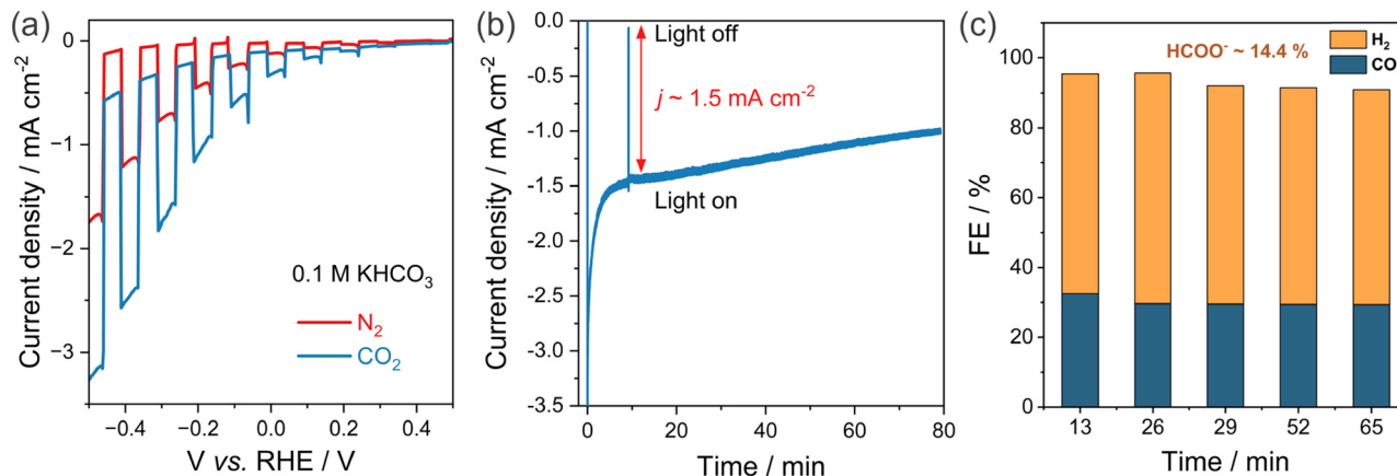
Fig. 3 PEC testing of the bare CIGS photocathode. (a) Current density vs. potential under 1 sun chopped light measured in N 2 - and CO 2 -saturated electrolyte. (b) Current density vs. time at -0.4 V vs. RHE for CO 2 -saturated electrolyte. (c) Time evolution of FE for CO and H 2 at -0.4 V vs. RHE. CO 2 saturated 0.1M KHCO 3 electrolyte, 1 sun simulated AM1.5G illumination. FE < 0.3% for gaseous products like methane and ethylene. FE < 1% for liquid products such as methanol, ethanol, and other C 2+ oxygenates.
