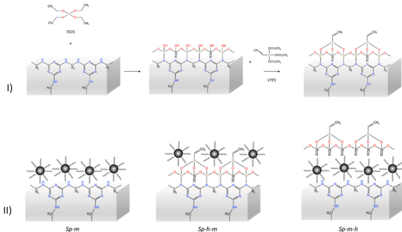
Scheme 1 Illustration of (I) the sol-gel process for the synthesis of hydrophobic coating and (II) the functionalized ligands (the representations of the ligands with curved lines) magnetic nanoparticles (black spheres) in either the pristine sponge or the organophilic sponges.
