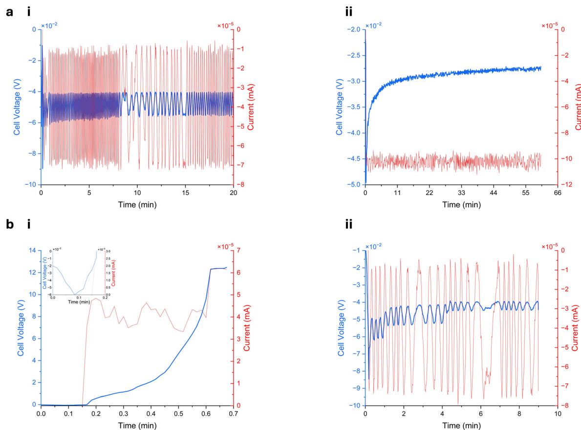
Fig. 2 Cycle graphs of sodiated regions. (a) Cycle graphs of sodium islands at different current densities (i) 0.04 \mu\text{A} \mu\text{m}^{-2} and (ii) 0.1 \mu\text{A} \mu\text{m}^{-2} . (b) Cycle graphs of a sodium island being cycled at 0.04 \mu\text{A} \mu\text{m}^{-2} ; the left-hand side shows the cell response of stripping sodium and the right-hand side shows the cell response of re-plating sodium. The inset of b(i) shows voltage response below the origin.
