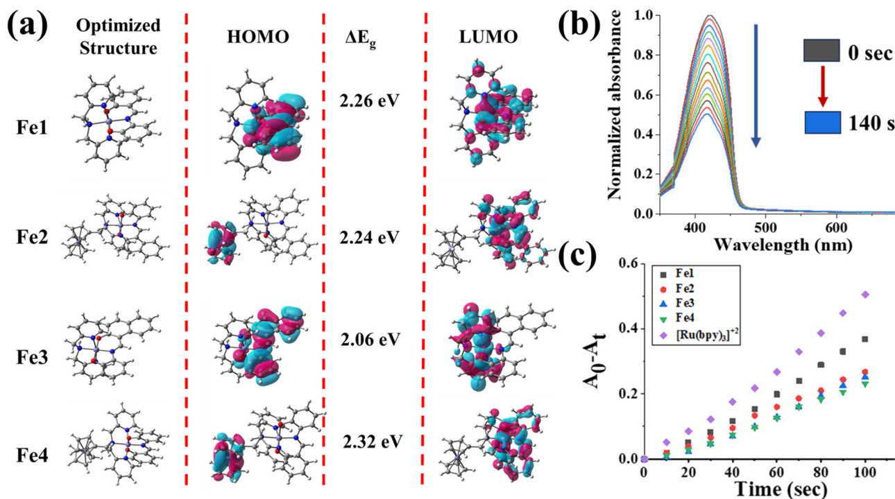
Fig. 2 (a) DFT energy-optimized structures, HOMO, LUMO of Fe1–Fe4 . (b) Singlet oxygen generation by Fe1 (10 μM) under visible light irradiation (400–700 nm, 10 J cm -2 ), monitored by the decrease in DPBF-based absorption peaks. (c) Comparison of 1 O 2 generation between Fe1–Fe4 and [Ru(bpy) 3 ]Cl 2 from the decline in the DPBF-based absorbance peak at 417 nm.
