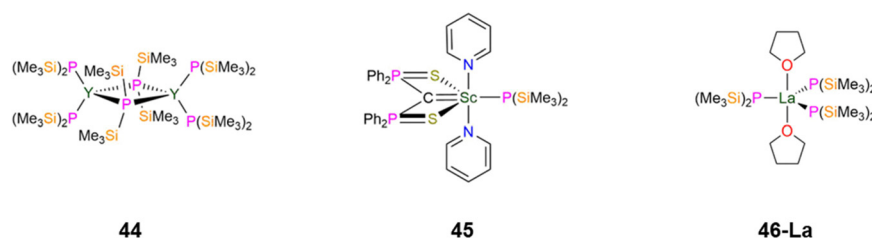
Fig. 13 Group 3 \text{P}'' complexes [\{\text{Y}(\text{P}'')_2(\mu\text{P}'')\}_2] ( 44 ), [\text{Sc}\{\text{C}(\text{PPh}_2\text{S})_2\}(\text{P}'')(\text{py})_2] ( 45 ), [\text{La}\{\text{P}(\text{SiMe}_3)_2\}_3(\text{THF})_2] ( 46-La ).
