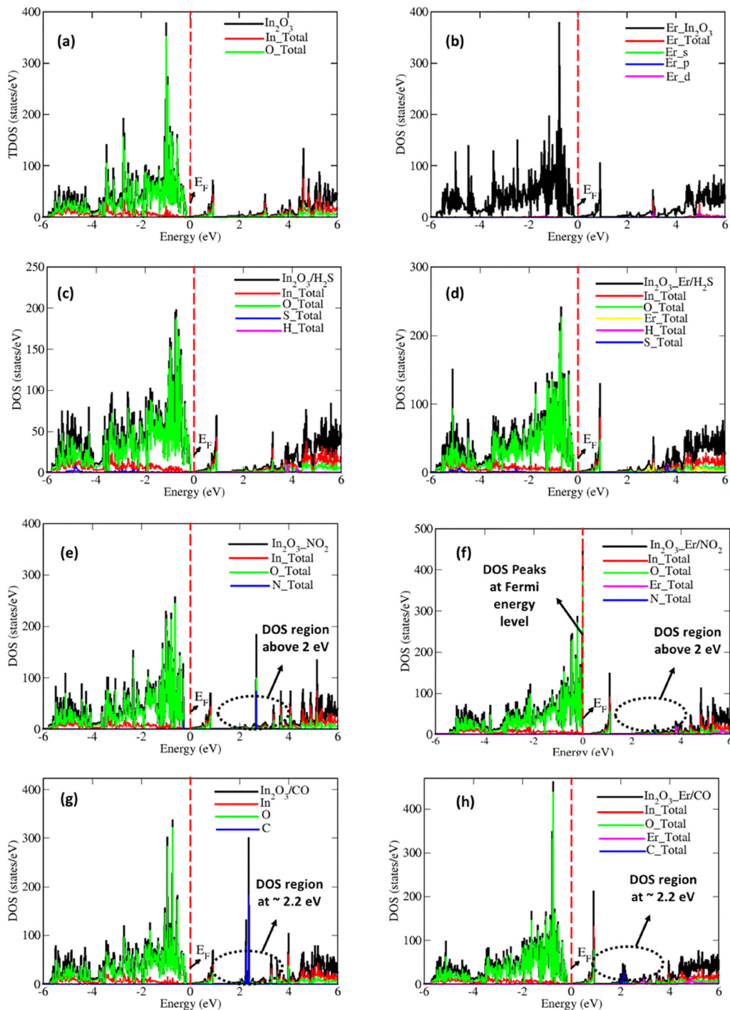
Fig. 4 Total and partial density of states (DOS and PDOS) of (a), (c), (e) and (g) pure and (b), (d), (f) and (h) Er-doped \text{In}_2\text{O}_3(001) surfaces: (a) and (b) without gas adsorption, (c) and (d) after \text{H}_2\text{S} adsorption, (e) and (f) after \text{NO}_2 adsorption, and (g) and (h) after \text{CO} adsorption. The red dotted line indicates the Fermi energy level.
