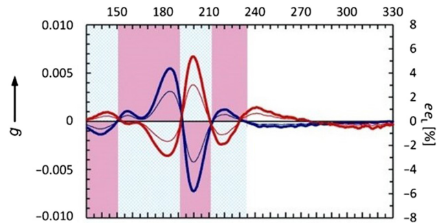
Fig. 3 Anisotropy spectra (thick lines) of isotropic amorphous D-Ala (red) and L-Ala (blue) in the vacuum-UV and UV spectral region. Thin lines represent the corresponding \epsilon_{\pm} plots inducible by either left or right circularly polarized light at \xi = 0.9999 . Amino acids were sublimated and condensed in the form of isotropic amorphous films. Reproduced and adapted from ref. 31 with permission from John Wiley and Sons, copyright 2012.
