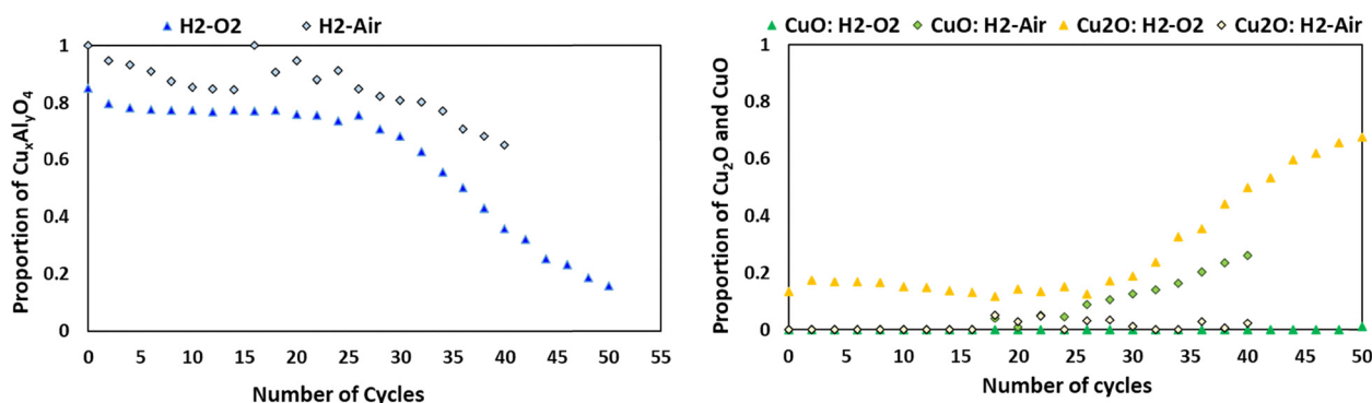
Fig. 6 Changes in the relative percentages of \text{Cu}_x\text{Al}_y\text{O}_4 (left) and \text{Cu}_2\text{O-CuO} phases (right) at the end of the oxidation reactions from fresh sample to up to 50 cycles for \text{H}_2\text{-O}_2 and \text{H}_2\text{-air} datasets.
