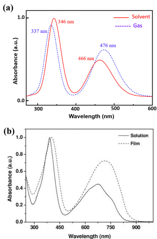
Fig. 8 (a) TD-DFT calculated UV-vis absorption spectra of PNDI-TV in chloroform solution and the gas phase. (b) Experimental data of UV-vis absorption spectra of PNDI-TV in chloroform solution and thin film taken from the work of Kim et al. 26 Reproduced with permission from WILEY.
