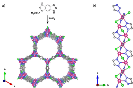
Fig. 1 (a) Crystal structure of \text{Co}_2\text{Cl}_2(\text{bbta}) viewed along the c -axis. (b) Structure of a helical cobalt-chloride-triazololate chain running along the c -axis (Co, pink; Cl, green; N, blue; C, grey; H, white).
