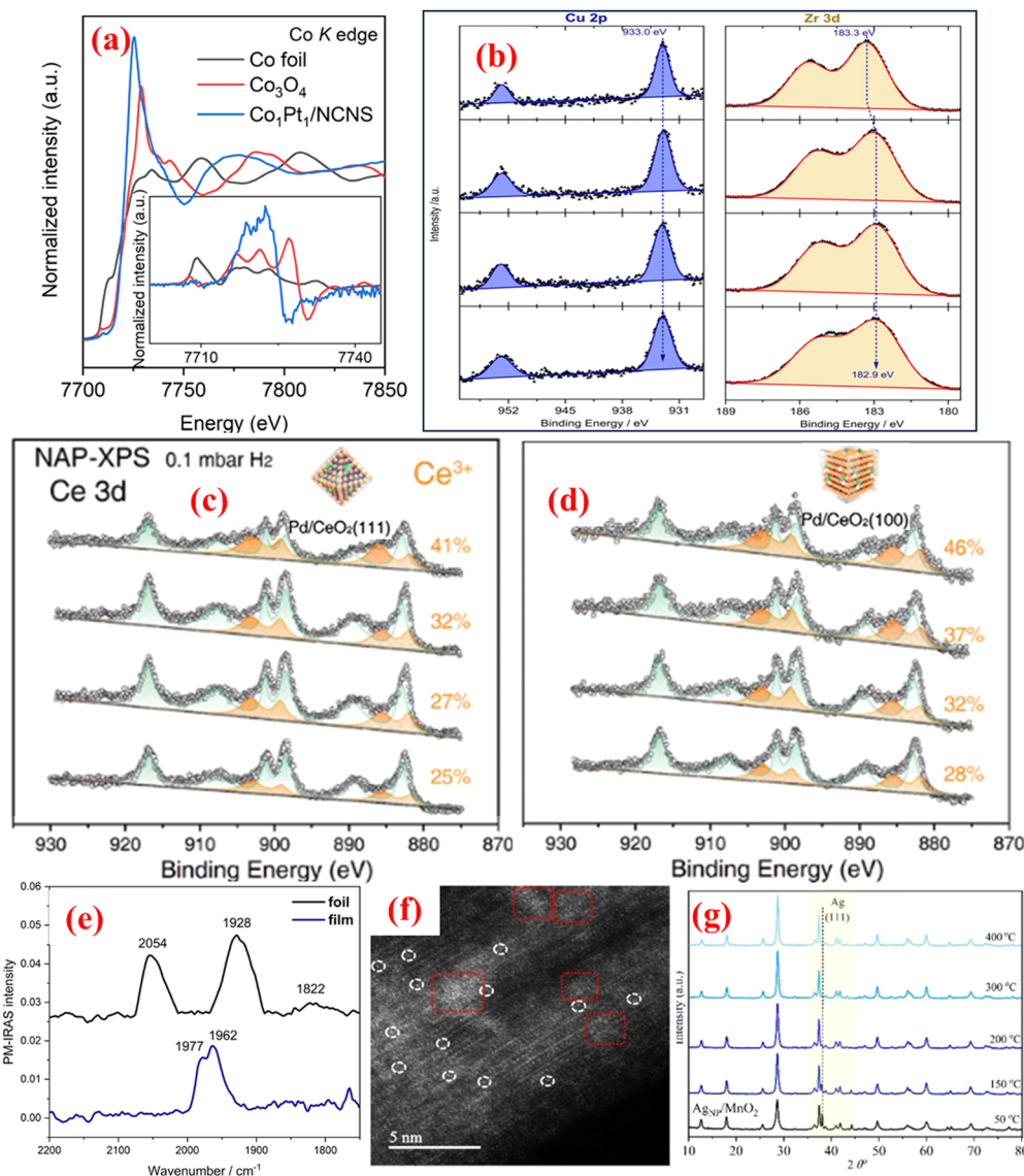
Fig. 3 (a) XANES spectra and first derivative curves (inset) of \text{Co}_1\text{Pt}_1 single atoms and reference samples. Reproduced with permission from ref. 31. Copyright 2021, Springer Nature. (b) NAP-XPS of Cu 2p and Zr 3d at 250 °C and 2 mbar in different reaction conditions. Reproduced with permission from ref. 37. Copyright 2024, Royal Society of Chemistry. NAP-XPS of Ce 3d in (c) Pd/CeO 2 (111) and (d) Pd/CeO 2 (100). Reproduced with permission from ref. 38. Copyright 2022, John Wiley and Sons. (e) PM-IRAS spectroscopy of CO adsorption over a Pd LCC catalyst. Reproduced with permission from ref. 39. Copyright 2024, Springer Nature. (f) HAADF-STEM image of AgNP/MnO 2 -350. Isolated Ag atoms are circled in white, Ag clusters in red rectangles. (g) In situ XRD patterns of AgNP/MnO 2 at distinct temperatures. Reproduced with permission from ref. 40. Copyright 2021, John Wiley and Sons.
