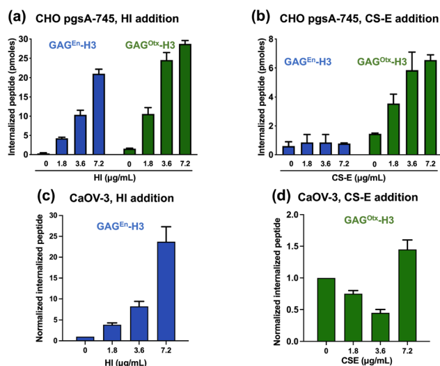
Fig. 7 MALDI-TOF MS quantification internalized GAG En -H3 or GAG Otx -H3 in pgsA-745 (a) and (b) or CaOV-3 (c) and (d) cells, incubated (7 μM) in the absence or presence of various concentrations of HI (a) and (c) or CS-E (b) and (d). In panels (a) and (b), the quantity of internalized peptides is given in pmoles; in panel (c) and (d), the internalization of the peptide in the presence of HI or CS-E is given relatively (normalized), to the quantity measured in the absence of the exogenously added GAGs.
