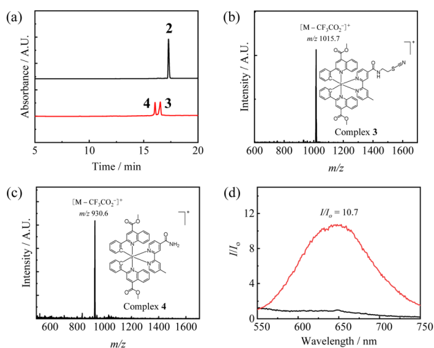
Fig. 1 (a) HPLC chromatograms of complex 2 (10 \mu M) in aerated PBS/DMSO (9 : 1, v/v) treated before (black) or after (red) photoirradiation. ESI-mass spectra of the photodissociation products collected at (b) t_R = 16.53 min and (c) t_R = 16.05 min of complex 2 (10 \mu M) in aerated PBS/DMSO (9 : 1, v/v) upon photoirradiation. (d) Emission spectra of complex 2 (10 \mu M) in aerated PBS/DMSO (9 : 1, v/v) treated before (black) or after (red) photoirradiation. Photoirradiation conditions for all experiments were carried out at 450 nm (10 mW cm -2 ) for 20 min at 298 K.
