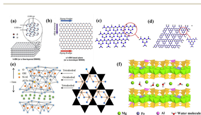
Fig. 2 (a) Layered van der Waals structure of bulk h-BN and (b) planar view of an atomically thin sheet of sp^2 -bonded B and N atoms that comprise the h-BN crystal or BN nanosheets (BNNS). Adapted with permission. 33 Copyright 2012, The Royal Society of Chemistry. Stacking 2D layering composition and fundamental constituent elements of (c) s-triazine and (d) tri-s-triazine of g\text{-C}_3\text{N}_4 . 34 Copyright 2017, Elsevier. (e) Schematic representation of the structure of MMT. 35 Copyright 2021, Multidisciplinary Digital Publishing Institute. (f) Schematic diagram of VMT structure. 19 Copyright 2021, Elsevier.
