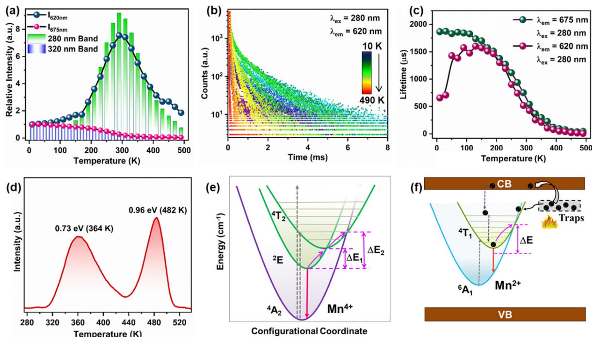
Fig. 3 (a) Variation in the peak intensity at 620 nm and 675 nm with temperature ( \lambda_{\text{ex}} = 280\text{ nm} ) and the CT band intensity for \lambda_{\text{em}} = 620\text{ nm} and 675 nm. (b) Luminescence decay profiles as a function of temperature at \lambda_{\text{ex}} = 280\text{ nm} and \lambda_{\text{em}} = 620\text{ nm} . (c) Temperature variation of lifetime for \lambda_{\text{ex}} = 280\text{ nm} . (d) TL spectra of YAGG:0.02Mn when irradiated with 280 nm light. (e) Schematic illustration of radiative transitions and possible thermal quenching mechanisms for Mn 4+ emission in octahedral coordination. (f) Schematic illustration of electron release from the traps and enhanced Mn 2+ emission with the increase in temperature.
