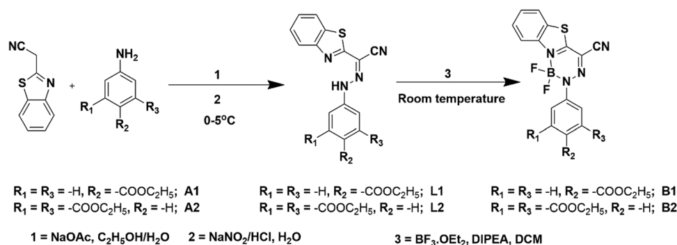
Scheme 1 Synthesis of ligands ( L1–L2 ) and BODIHYs ( B1–B2 ).
