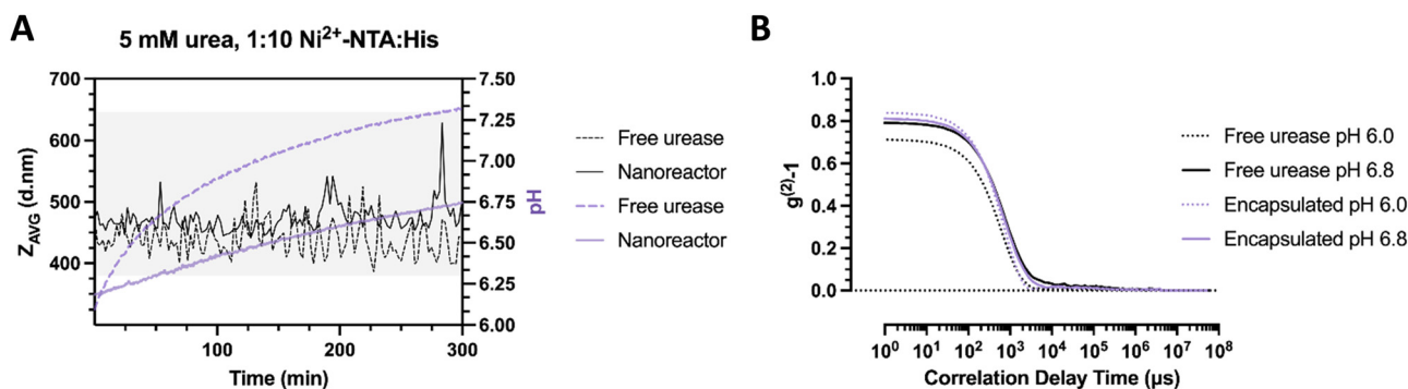
Fig. 6 (A) pH evolution and Z AVG of clustering stomatocytes measured over time (5 mM urea) with urease encapsulated in the nanoreactors or free (0.1 nM urease by Nanodrop analysis) in solution. (B) Associated correlation curves of clustering stomatocytes with free or encapsulated urease at pH 6.0 and 6.8.
