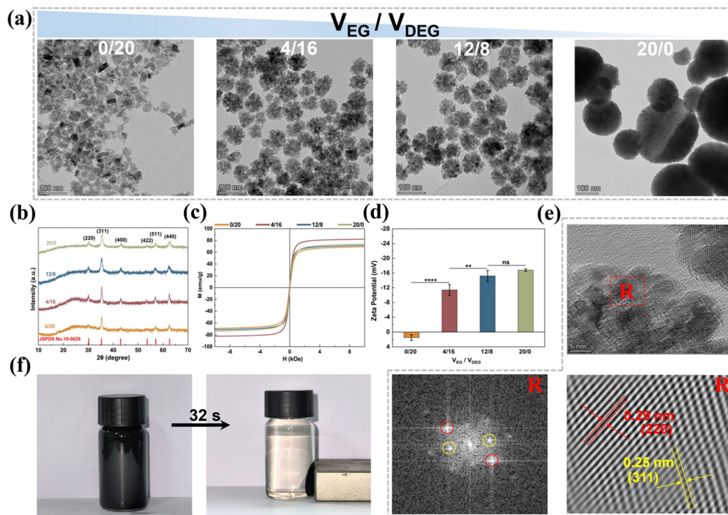
Fig. 2 Characterization of MNPs synthesized with different V_{EG}/V_{DEG} ratios. (a)–(d) TEM images (a), XRD spectra (b), M-H curves (c), and zeta potential (d) of MNPs synthesized with V_{EG}/V_{DEG} ratios of 0/20, 4/16, 12/8, and 20/0. (e) HRTEM images of MNPs synthesized with V_{EG}/V_{DEG} ratio of 4/16. (f) Digital photos of MNPs dispersed in water (left) and collected by magnetic separation (right).
