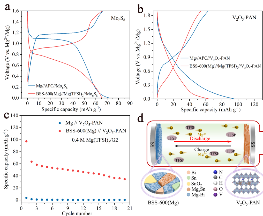
Fig. 8 Full-cell discharge/charge curves for the (a) Mo 6 S 8 and (b) V 2 O 5 -PAN cathode system at 50 mA g -1 . (c) Comparison of cycling performance of the Mg//V 2 O 5 -PAN and BSS-600(Mg)//V 2 O 5 -PAN full cells using Mg(TFSI) 2 /G2 electrolyte. (d) Schematic diagram of the full cell with a BSS-600 anode of the rechargeable magnesium batteries.
