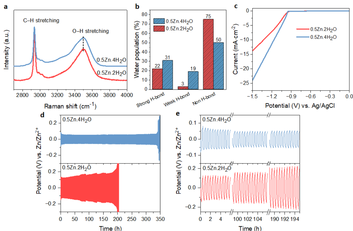
Fig. 6 Solvation structure and electrochemical stability of the Zn anode in 0.5\text{Zn}\cdot 4\text{H}_2\text{O} electrolyte compared to concentrated 0.5\text{Zn}\cdot 2\text{H}_2\text{O} . (a) Raman spectra in the water region. (b) The corresponding water population percentages. (c) LSV curves on a Ti substrate (d) Zn plating/stripping at 2\text{ mA cm}^{-2} and 0.5\text{ mA h cm}^{-2} in \text{Zn}||\text{Zn} symmetric cells and (e) the corresponding potential profiles.
