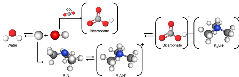
Fig. 7 Representation of the process of CO 2 capture by tertiary amines.
