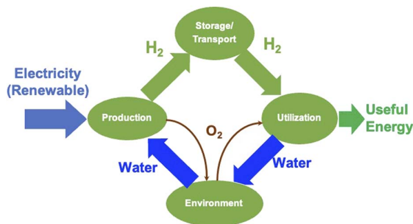
Fig. 4 Splitting of water (H 2 O) using renewable electricity is a net-zero emission process and is also circular in nature, becoming completely sustainable. This is because the product of H 2 combustion will produce H 2 O, which can be reused if collected at the source and recovered completely. This process can be least harmful both environmentally and ecologically.
